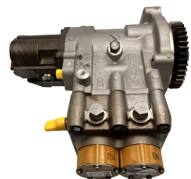
Model:511-7975柴油泵
