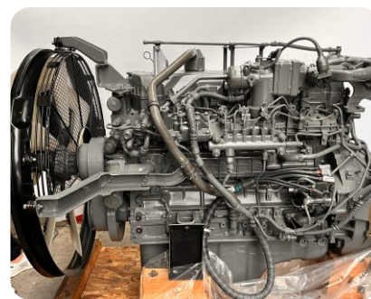
Engine:6HK1
